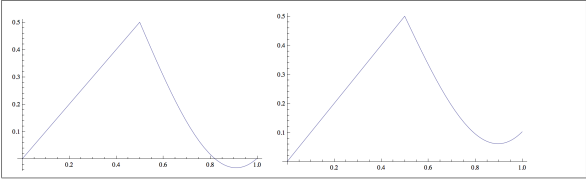
Figure 1: Utilities of users using strategies (x, x) under \lambda and \lambda' .
