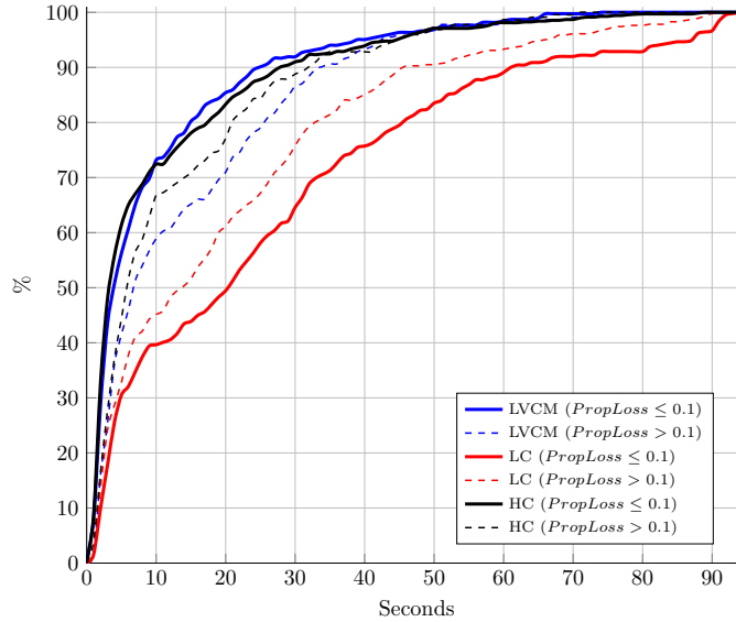
Figure 5.4: Response-Time Frequencies
